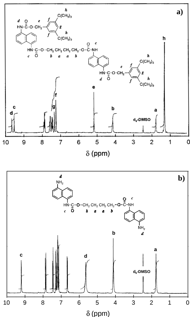
Fig. 1 ^1\text{H} NMR spectra ( \text{d}_6\text{-DMSO} as solvent) of a) the 3,5-di- t BBOC terminated compound 19 (oligourethane 1e with n=1 ) and b) the corresponding amino terminated compound 20 (oligourethane 1a with n=1 ) after cleavage of the protective group
